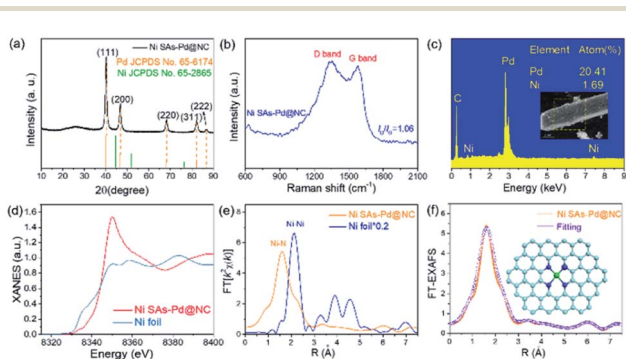
Fig. 3 Structural characteristics of Ni SAs-Pd@NC. (a) XRD pattern. (b) Raman spectrum. (c) EDX analysis. (d) XANES spectra of the Ni K-edge. (e) FT-EXAFS of the Ni K-edge. (f) EXAFS fitting curves at the R space (inset: atomic structure model of Ni sites).
