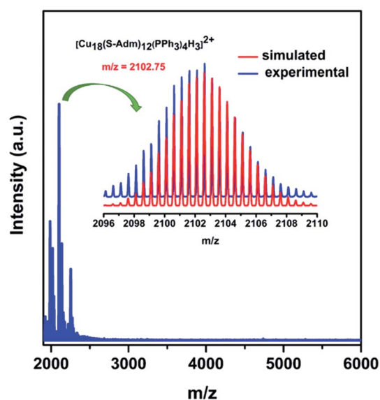
Fig. 4 Positive-mode ESI-MS spectrum of Cu_{18} NC over the m/z range of 1900 to 6000. Inset shows the experimental and simulated patterns of the peak corresponding to [Cu_{18}(S-Adm)_{12}(PPh_3)_4H_3]^{2+} .
