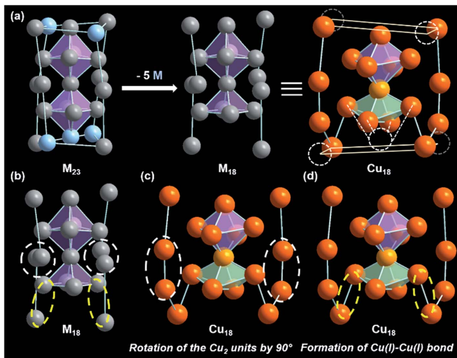
Fig. 3 (a) Metallic skeleton of the Ag_{23} NC, which is denoted here as M_{23} , and that of Cu_{18} NC with five metal vacancy positions, which is similar to that of M_{18} . (b) Metallic skeleton of perfect M_{18} with the positions at which reconstruction happened for Cu_{18} marked. (c) Rotation of the two Cu_2 units in the metal–ligand motifs of Cu_{18} NC, and (d) formation of Cu(I)-Cu(I) bonds. Color legend: Cu, light and deep orange; Ag, grey and sky blue.
