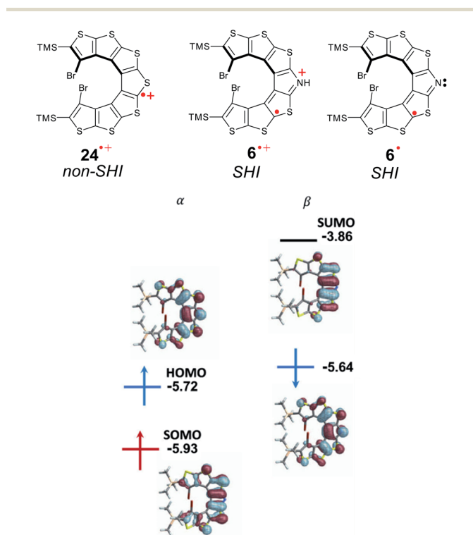
Fig. 16 Chemical structures of cationic radicals thia[7]helicene 24^{+\bullet}[PF_6]^{-} and aza-thia[7]helicene 6^{+\bullet}[PF_6]^{-} , and neutral aza-thia[7]helicene 6^{\bullet} . Orbital energies (in eV) and isosurfaces ( \pm 0.030 a.u.) of selected MOs of 7 . Figures adapted with permission from ref. 53. Copyright 2021 American Chemical Society.
