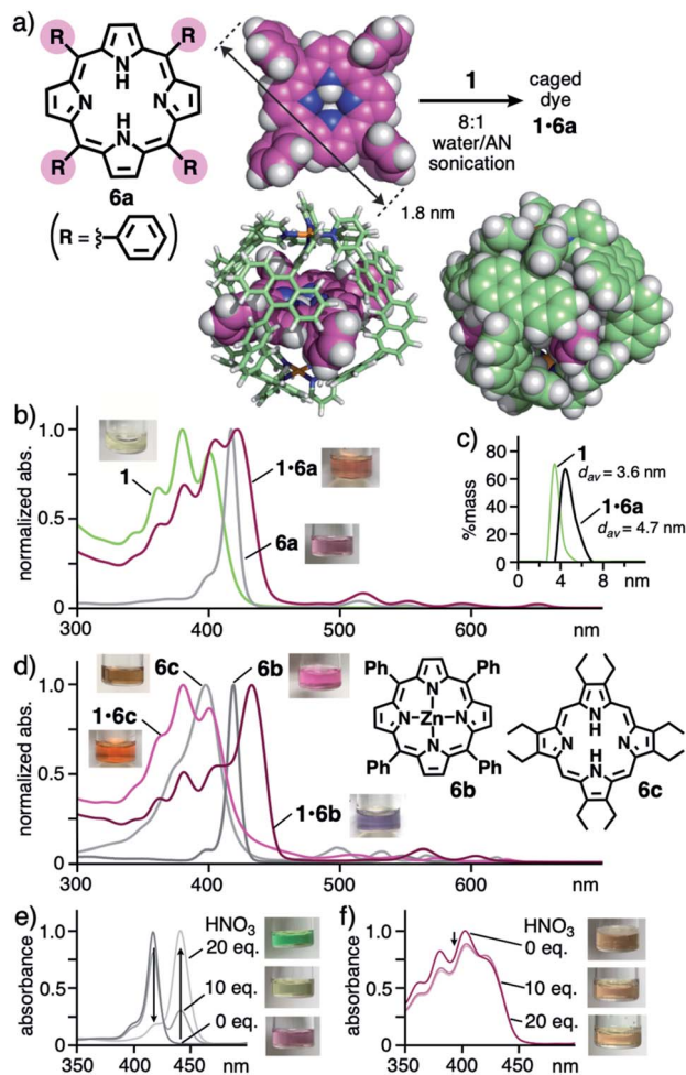
Fig. 6 (a) Formation of caged dye 1·6a and the optimized structures of 6a and 1·6a ( R^1 = H for clarity). 11 (b) UV-visible spectra and photographs (8 : 1 water/AN, r.t.) of 1·6a , 1 , and 6a (in CH_2Cl_2 ) and (c) their DLS charts (r.t.) except for 6a . (d) UV-visible spectra and photographs (8 : 1 water/AN, r.t.) of 1·6b , 1·6c , and 6b , 6c (in CH_2Cl_2 ). UV-visible spectra and photographs (r.t.) of (e) 6a in CH_2Cl_2 and (f) 1·6a in 8 : 1 water/AN, after addition of HNO_3 (0–20 equivalents).
