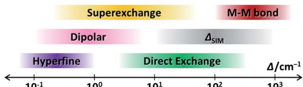
Fig. 11 The schematic representation of the energy ranges that the discussed magnetic couplings usually affect, along with the single-ion \Delta_{\text{SIM}} , in a lanthanide-based SMM.
