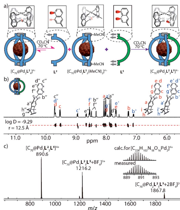
Fig. 3 Self-assembly and characterization of heteroleptic cage [\text{C}_{70}@\text{Pd}_2\text{L}_3\text{L}^5]^{4+} : (a) when bowl [\text{C}_{70}@\text{Pd}_2\text{L}_3(\text{MeCN})_2] reacts with ligand \text{L}^2 or \text{L}^5 in a 1 : 1 ratio at 70^\circ\text{C} , the former ligand only yields minor amounts of cage [\text{Pd}_2\text{L}_4] while the latter leads to quantitative conversion; (b) ^1\text{H} NMR and DOSY spectra (600 MHz, 298 K, \text{CD}_3\text{CN} ) of cage [\text{C}_{70}@\text{Pd}_2\text{L}_3\text{L}^5] (0.64 mM); (c) high-resolution ESI mass spectrum of [\text{C}_{70}@\text{Pd}_2\text{L}_3\text{L}^5] and \text{BF}_4^- adducts.
