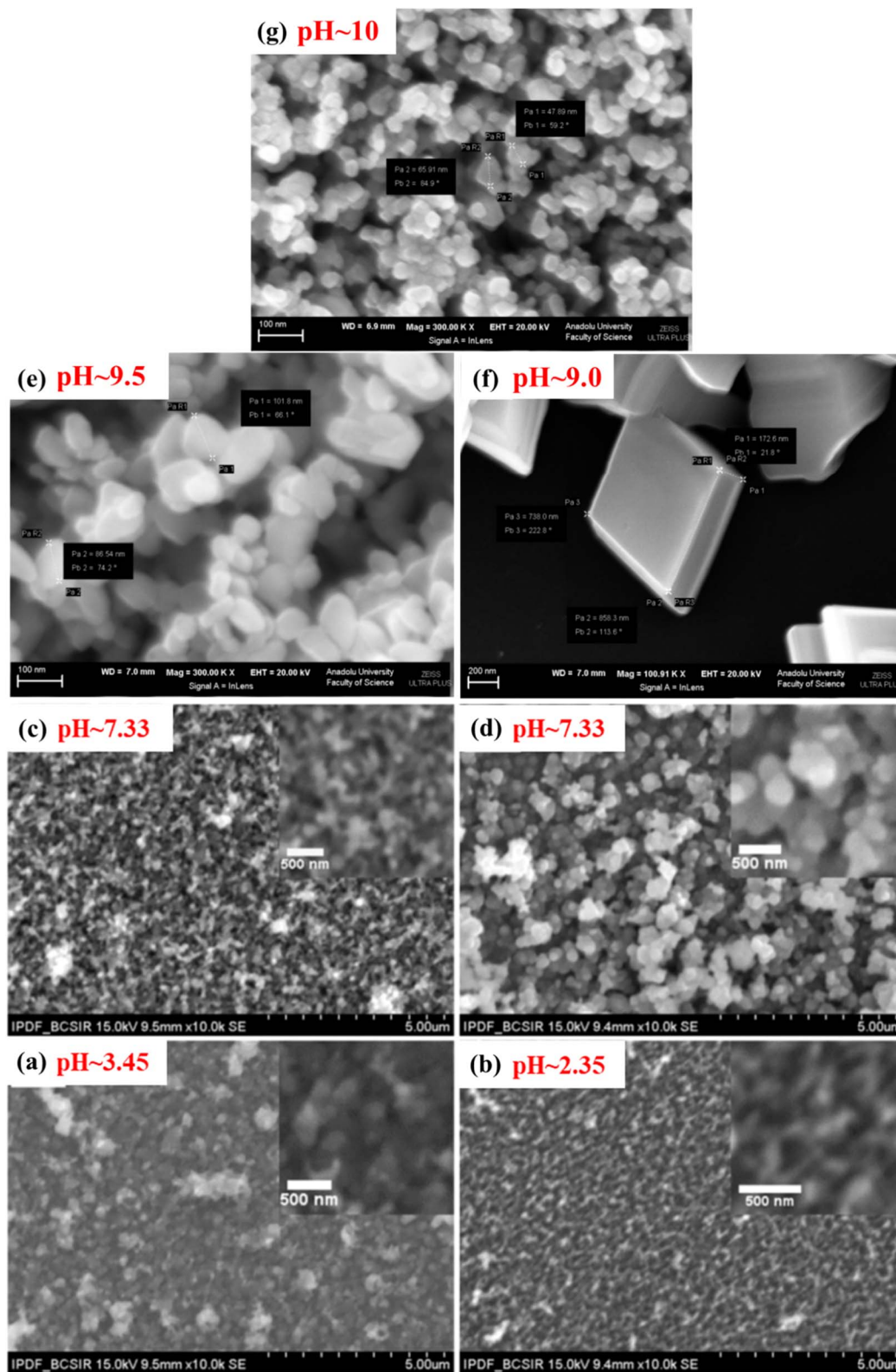
Fig. 6 SEM images representing {Cu 2 O: (a)–(d) and CuO: (e)–(g)} thin films deposited by varying pH. 36,105
