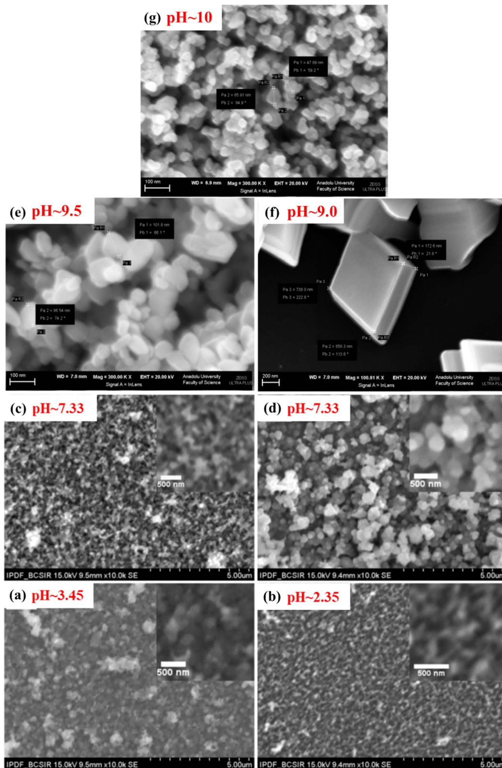
Fig. 6 SEM images representing {Cu 2 O: (a)–(d) and CuO: (e)–(g)} thin films deposited by varying pH. 36,105
