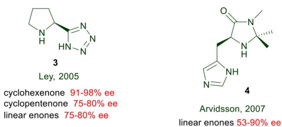
Scheme 4 Conjugate additions using pyrrolidines and imidazolide catalysts.
