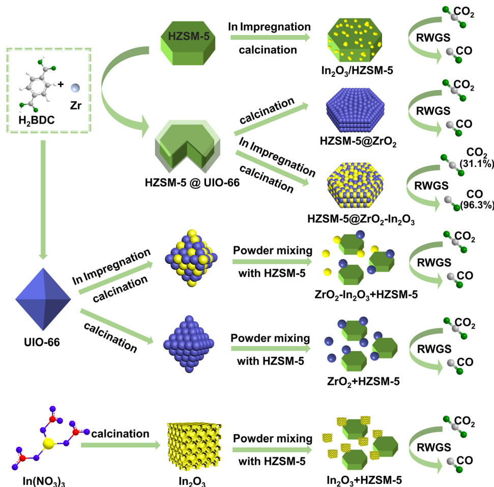
Fig. 1 Assembly diagram of composites (from top to bottom) In 2 O 3 /HZSM-5, HZSM-5@ZrO 2 , HZSM-5@ZrO 2 -In 2 O 3 , ZrO 2 -In 2 O 3 + HZSM-5, ZrO 2 + HZSM-5, In 2 O 3 + HZSM-5 and their effects on CO 2 hydrogenation.
