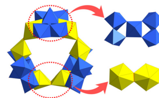
Fig. 27 View of \{[\text{W}_5\text{O}_{21}]_3[(\text{U}^{\text{VI}}\text{O}_2)_2(\mu\text{-O}_2)]_3\}^{30-} . Color codes are the same as in Fig. 1.
