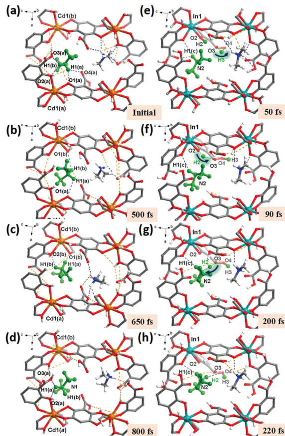
Fig. 4 Migration trajectory of \text{Me}_2\text{NH}_2^+ in Cd-BQ-COOH at (a) the initial state; (b and c) the intermediate states; and (d) the later state. (e and f) The pathway of proton hopping between the -\text{OH} group and -\text{COOH} group in In-BQ-COOH . (g) A strong interaction is established between the \text{H}^+ and \text{Me}_2\text{NH} . (h) Formation of a protonated \text{Me}_2\text{NH}_2^+ . Note: The \text{Me}_2\text{NH}/\text{Me}_2\text{NH}_2^+ and the hopping protons are highlighted in green. The blue and orange dashed lines illustrate the changes of \text{N}\cdots\text{O} and \text{O}\cdots\text{H}\cdots\text{O} bonds, respectively.
