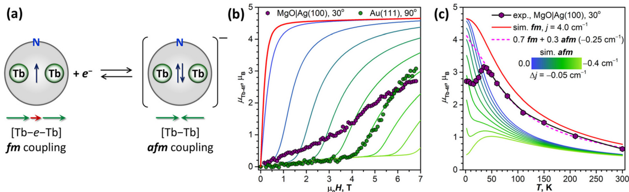
Fig. 10 (a) Schematic description of the electron trapping by the SOMO of \text{Tb}_2@C_{79}\text{N} leading to \text{Tb}_2@C_{79}\text{N}^- anion with two-fold occupied \text{Tb}-\text{Tb} bonding MO and antiferromagnetic coupling of magnetic moments; green arrows denote \text{Tb-4f} magnetic moments, red arrow denotes magnetic moment of the unpaired valence electron. (b) Magnetization curves of \text{Tb}_2@C_{79}\text{N} on \text{MgO}|\text{Ag}(100) and \text{Au}(111) measured at T \approx 2\text{ K} and compared to the results of simulations for fm and afm coupling of \text{Tb-4f} magnetic moments, the coloring scheme is the same as in (c). (c) Temperature dependence of \text{Tb-4f} magnetic moment in \text{Tb}_2@C_{79}\text{N} 1.5 ML on \text{MgO}|\text{Ag}(100) measured by XMCD at 6.8\text{ T} in grazing incidence and compared to the results of simulations for ferromagnetic (fm) and antiferromagnetic (afm) coupling of \text{Tb-4f} magnetic moments with different values of the coupling constant j_{12} ; dashed line is a simulation for a mixture of molecules with fm (70%) and afm (30%) ground states.
