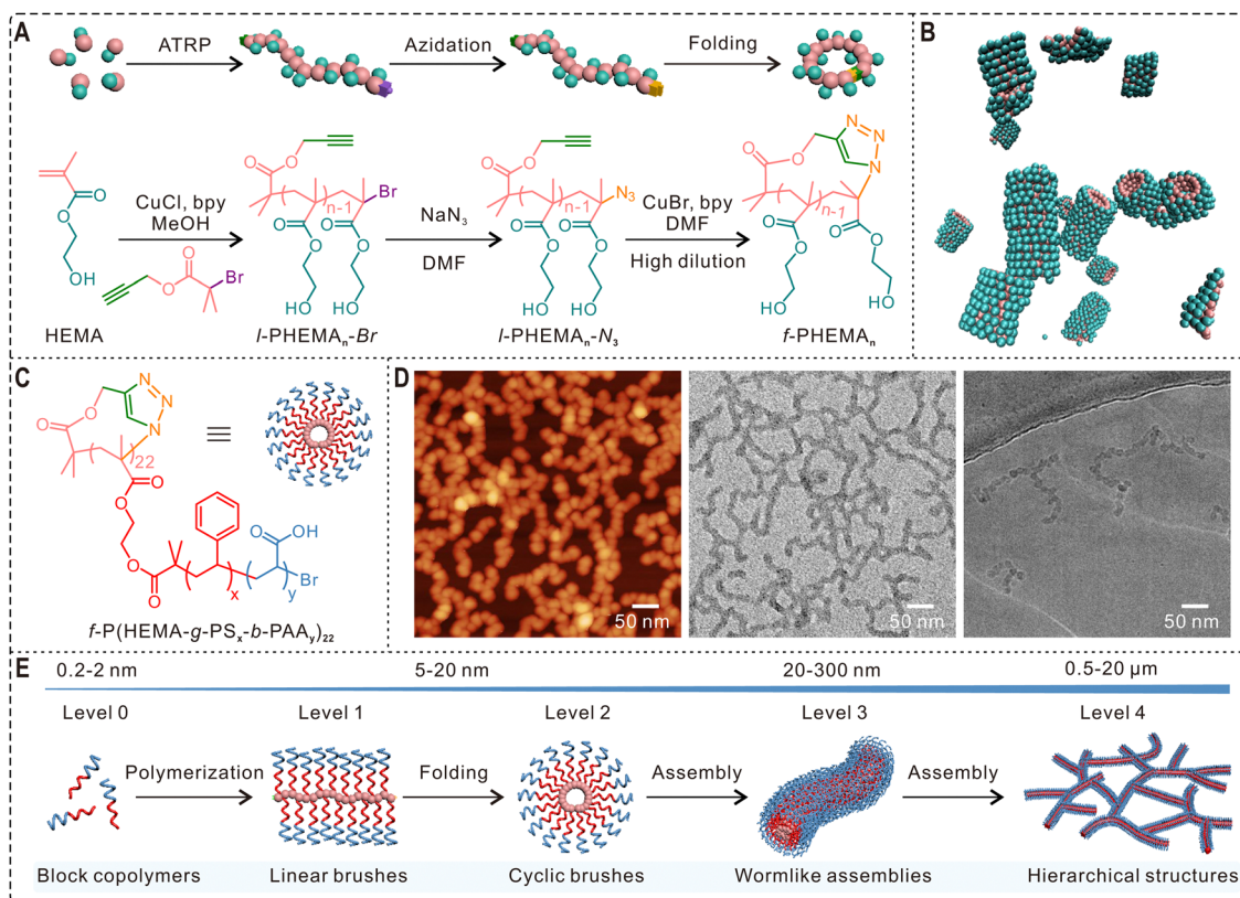
Fig. 4 Hierarchical nanostructures self-assembled from cyclic polymers. (A) Scheme of the synthesis of I\text{-PHEMA}_n\text{-Br} and its azidation and folding into the cyclic topology. (B) Molecular dynamic simulation snapshot showing the self-assembly of f\text{-PHEMA}_{15} into wormlike structures. (C) Molecular structure and scheme of cyclic brush polymer f\text{-P(HEMA-g-PS}_x\text{-b-PAA}_y\text{)}_{22} . (D) AFM (left), TEM (middle), and cryo-TEM (right) images showing the self-assembly of cyclic brush polymers into 1D wormlike assemblies and hierarchical structures at 0.4 \text{ mg mL}^{-1} in water. (E) Schematic of the formation of hierarchical structures by synthetic polymers via biomimetic folding and self-assembly. Copyright 2021 The Authors. Reproduced with permission. 32 Published by Springer Nature.
