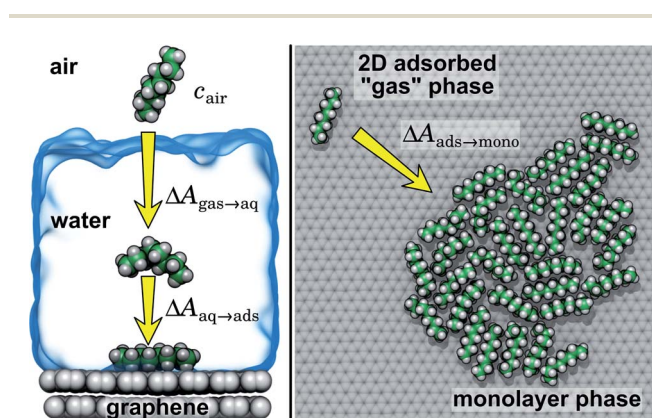
Fig. 3 Diagram of free-energy changes for adsorption of alkanes to the graphene–water interface from air. \Delta A_{\text{gas} \rightarrow \text{aq}} is the hydration free energy. \Delta A_{\text{aq} \rightarrow \text{ads}} is the free energy for single-molecule adsorption from the aqueous phase to the graphene–water interface. \Delta A_{\text{ads} \rightarrow \text{mono}} is the free energy for condensing from the 2D gas phase to the bulk of the monolayer condensed phase.
