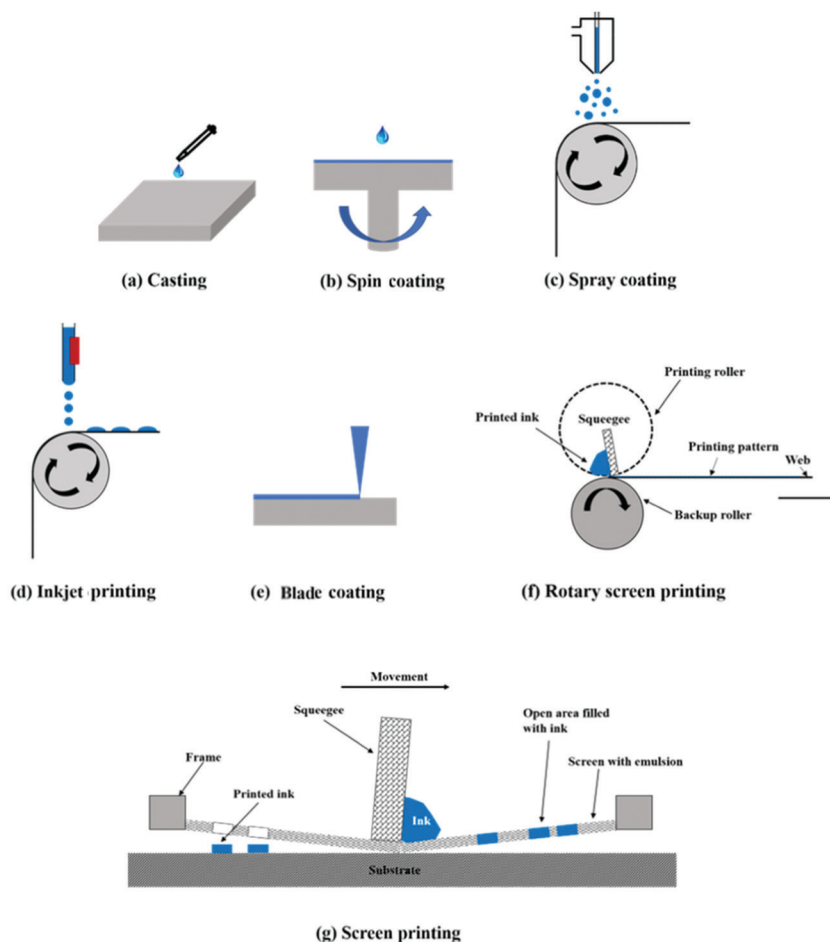
Fig. 1 Single substrate-based fabrication technologies. Reproduced with permission. 47 Copyright 2020, the authors, under the Creative Commons Attribution 3.0 license (c and d). Reproduced with permission. 45 Copyright 2009, Elsevier (f and g).
