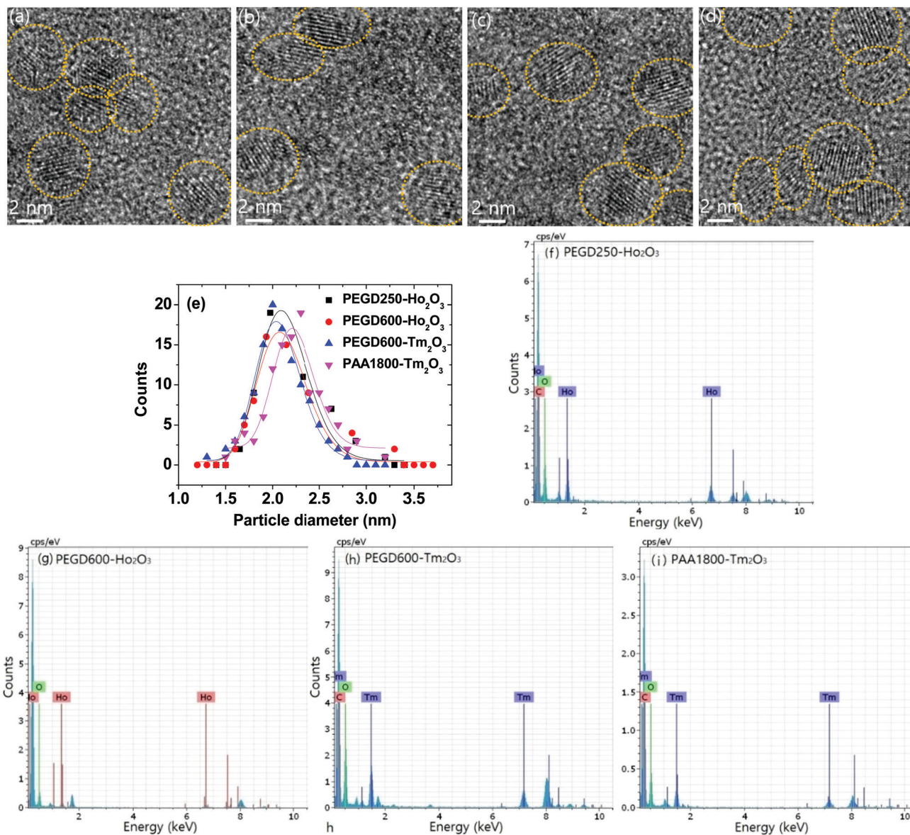
Fig. 1 HRTEM images of (a) PEGD250- and (b) PEGD600-coated ultrasml \text{Ho}_2\text{O}_3 nanoparticles and (c) PEGD600- and (d) PAA1800-coated ultrasml \text{Tm}_2\text{O}_3 nanoparticles. (e) Log-normal function fits to the observed particle diameter distributions to obtain d_{\text{avg}} . EDS spectra of (f) PEGD250- and (g) PEGD600-coated ultrasml \text{Ho}_2\text{O}_3 nanoparticles and (h) PEGD600- and (i) PAA1800-coated ultrasml \text{Tm}_2\text{O}_3 nanoparticles.
