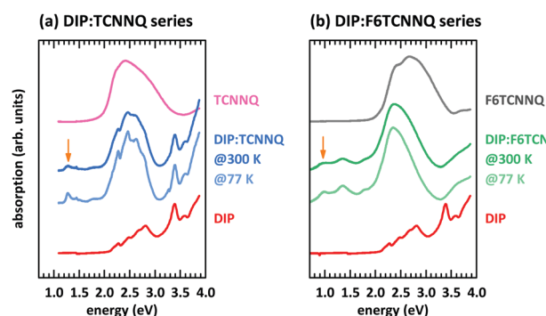
Fig. 4 Absorption spectra for single component and equimolar co-deposited D:A films of DIP and TCNNQ (a) as well as of DIP and F6TCNNQ (b). The CT transitions are marked by orange arrows. The absorption spectra for co-deposited D:A were measured at 300 K and at 77 K.
