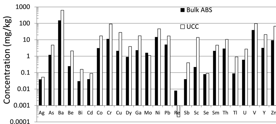
Fig. 2 Abundance of TE in bulk ABS and UCC. Concentration data for ABS from Bicalho et al. 39 except for Se. 27 Data for the UCC from Rudnick and Gao. 40
