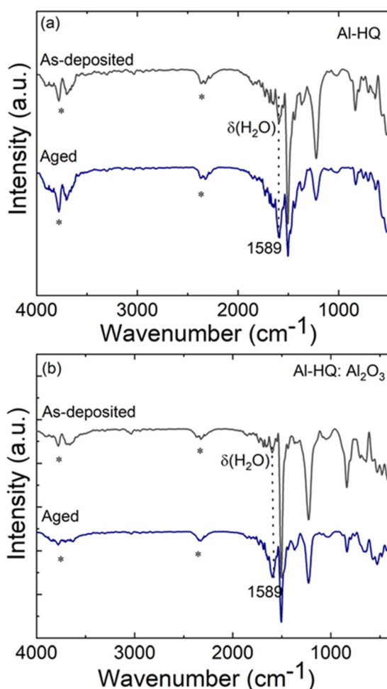
Fig. 3 Stability studies of Al-HQ films: FTIR spectra for (a) a 70 nm thick Al-HQ film immediately after the deposition and aging (two-week) in ambient conditions, and (b) Al-HQ film deposited at 140\text{ }^\circ\text{C} and capped with 45 nm \text{Al}_2\text{O}_3 layer measured immediately after the deposition and after one-week storage in ambient conditions. The bands marked with * are caused by adsorbed \text{CO}_2 .
