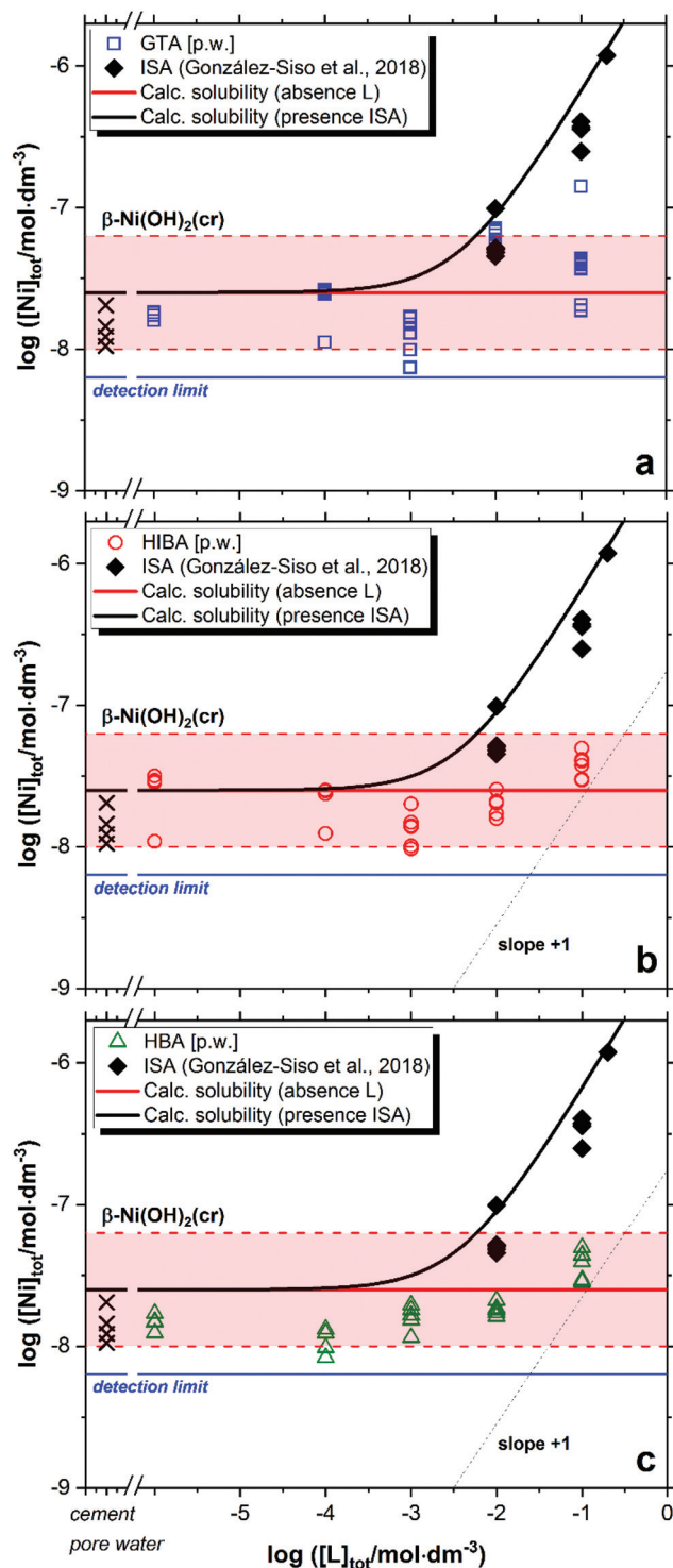
Fig. 3 Solubility of \beta\text{-Ni(OH)}_2(\text{cr}) in equilibrium with cement porewater at \text{pH} = 12.5 with 10^{-6} \text{ M} \leq [\text{L}]_{\text{tot}} \leq 0.1 \text{ M} at t \leq 359 days: (a) glutaric acid (GTA); (b) \alpha -hydroxyisobutyric acid (HIBA); (c) 3-hydroxybutyric acid (HBA). Cross symbols show the concentration of \text{Ni(II)} determined in cement porewater. Red solid and dashed lines in the figure represent the calculated solubility of \beta\text{-Ni(OH)}_2(\text{cr}) and corresponding uncertainty at \text{pH} = 12.5 in ligand-free systems. Black lines correspond to the solubility of \beta\text{-Ni(OH)}_2(\text{cr}) in the presence of ISA. All thermodynamic calculations performed using the chemical and thermodynamic models reported in González-Siso et al. (2018). 51
