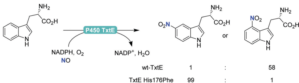
Scheme 21 Regioselective nitration of tryptophan with the P450 monoxygenase from Streptomyces scabies (P450 TxtE) and one of its mutants.
