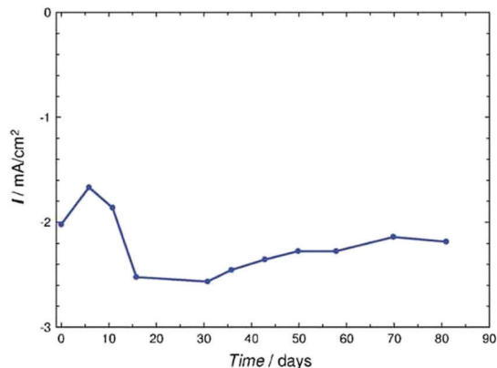
Fig. 94 Schematic of PEDOT-based HER electrode (left side). Long-term performance of PEDOT-PEG on Goretex/Au in 1 M H 2 SO 4 under N 2 at -0.35 V vs. SCE. Reproduced with permission from ref. 1339. Copyright 2010 Wiley.
