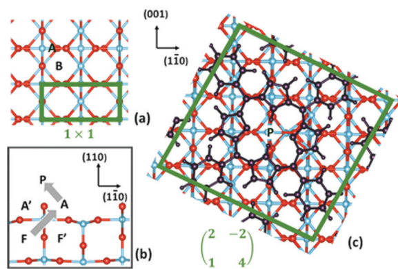
Fig. 14 (a) Top and (b) side views of the \text{TiO}_2(110) surface; and (c) top view of the oblique supercell used in the present work, where the adsorbed 2H-TPP film is also shown. Relevant sites for Ti are indicated. Ti atoms are blue, O atoms are red, and all the 2H-TPP atoms are black. The borders of the (1 \times 1) unit cell and of the oblique supercell are marked with green lines. The grey arrows in (b) show the approximate path of Ti during the self-metalation reaction. Reproduced from ref. 48 with permission from Elsevier, Copyright 2021.
