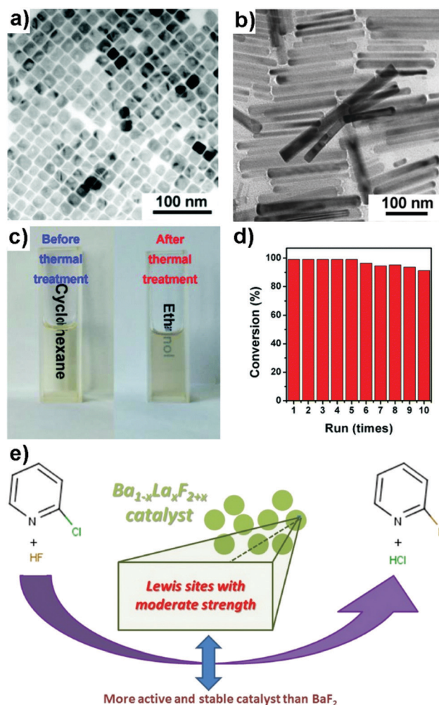
Fig. 6 TEM images of (a) \text{NaScF}_4 and (b) \text{KSc}_2\text{F}_7 nanocrystals. (c) Photograph of \text{NaScF}_4 nanocrystal solutions before and after thermal treatment at 500 °C under Ar/ \text{H}_2 . (d) Reusability test of \text{NaScF}_4 nanocrystals for 10 cycles in the cyanosilylation reaction. 96 Reprinted with permission from ref. 96. Copyright 2017, Royal Society of Chemistry. (e) A scheme for the gas phase fluorination of 2-chloropyridine by HF using \text{Ba}_{1-x}\text{La}_x\text{F}_{2+x} . 97 Reprinted with permission from ref. 97. Copyright 2017, Elsevier.
