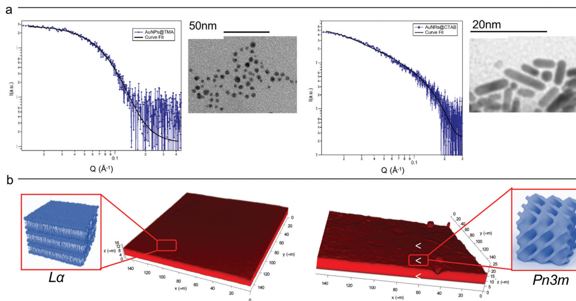
Fig. 1 (Panel a) Physicochemical properties of NPs. Left: SAXS profile of AuNSs in water (at a concentration of 1.1 \times 10^{15} particles mL -1 ) and the corresponding fit with a Schulz polydisperse spheres model (see ESI,† for details). The inset shows a typical TEM image of AuNSs; Right: SAXS profile of AuNRs in water (at a concentration of 2.4 \times 10^{14} particles mL -1 ) and curve fitting according to a Cylinder poly radius model. The inset reports a TEM image of AuNRs; (Panel b) physicochemical properties of lipid films. Three-dimensional reconstruction of a confocal fluorescence z-stack of images of the lamellar (left side) and the cubic (right side) films (tilted surface area of 150 \times 150 \mu\text{m} ). The insets depict the lamellar L\alpha (left side) and cubic Pn3m (right side) structures.
