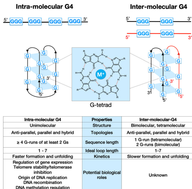
Fig. 1 Schematic representation of intra- and inter-molecular G-quadruplex (G4) structures and their properties. A planar G-tetrad structure is formed by four guanines stabilised by Hoogsteen hydrogen bonds and coordinated by a central monovalent cation. Intra-molecular G4s are formed within a single DNA strand, while inter-molecular G4s generate from two (or more) strands.
