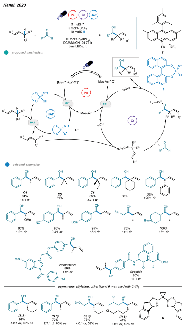
Scheme 14 Photoredox and chromium dual-catalyzed allylation of aldehydes using unactivated alkenes.
