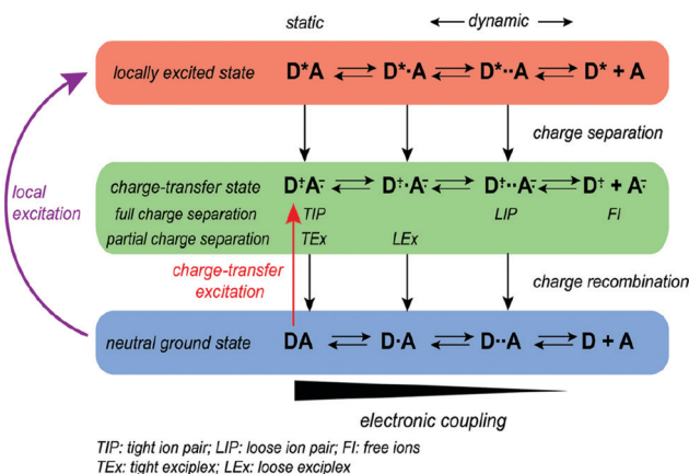
Fig. 2 Donor and acceptor charge transfer schemes in polar solvents. Reprinted with permission from ref. 29. Copyright 2017 American Chemical Society.
