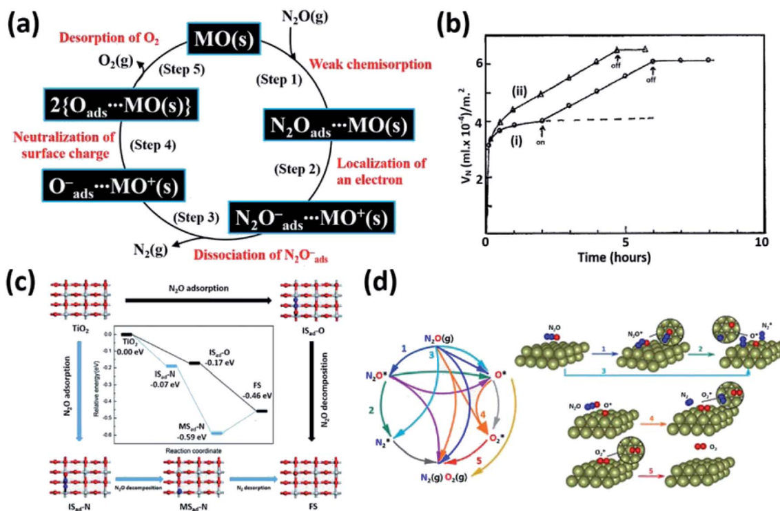
Fig. 12 (a) Mechanism of the conversion of \text{N}_2\text{O} to \text{N}_2 and \text{O}_2 over a metal oxide surface. (b) Time-dependent production of \text{N}_2 ( V_N ) from \text{N}_2\text{O} (10 Torr) over an activated ZnO surface at 20 °C under (i) dark and light on/off conditions indicated by arrows and (ii) continuous illumination. Reprinted with permission from ref. 152. Copyright© 1971, American Chemical Society. (c) Relative energy diagram for the photocatalytic decomposition of \text{N}_2\text{O} on perfect anatase (001) facets. Reprinted with permission from ref. 173. Copyright© 2018, Royal Society of Chemistry. (d) Reaction diagram for the conversion of \text{N}_2\text{O} to various adsorption and decomposition products ( \text{N}_2\text{O}^* , \text{N}_2^* , \text{O}^* , \text{O}_2^* , \text{N}_2(\text{g}) and \text{O}_2(\text{g}) ; * designates adsorbed species). (1–3) Dissociative adsorption of \text{N}_2\text{O} on Ir(111), (4) formation of surface peroxides, and (5) \text{O}_2 desorption from Ir(111). Reprinted with permission from ref. 177. Copyright© 2019, American Chemical Society.
