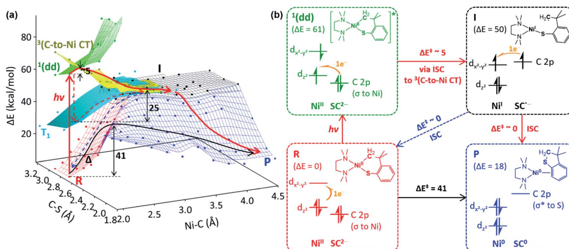
Fig. 5 (a) The ground- and excited-state PESs of 1 tmeda , colored according to the electronic configurations of the ground state (red) and the ^1(\text{dd}) (green), ^3(\text{C-to-Ni CT}) (yellow), and T 1 (cyan) excited states of the Ni II (SC 2- ) reactant ( R ), the Ni I (SC - ) intermediate ( I , black), and the Ni 0 + SC 0 product ( P , blue). A plausible photo-induced RE pathway from the ^1(\text{dd}) state and the dark RE pathway are drawn with red and black solid arrows, respectively. Alternative paths are noted with dashed arrows. (b) Electronic configuration and potential energy (in kcal mol -1 ) changes over the reactions presented in (a).
