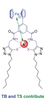
Fig. 6 Schematic representation of through-bond (TB, blue) and through-space (TS, green arrows) interactions that drive anion recognition in the cationic state of 1.XB/HB in solution and at 2.XB/HB SAM . In the more polar solvent environment of high dielectric the TS contribution is diminished and TB contributions are significant. In the low dielectric SAM environment, TS contributions are strongly enhanced such that binding in the cationic state is switched-on more strongly, inducing a larger sensor response.
