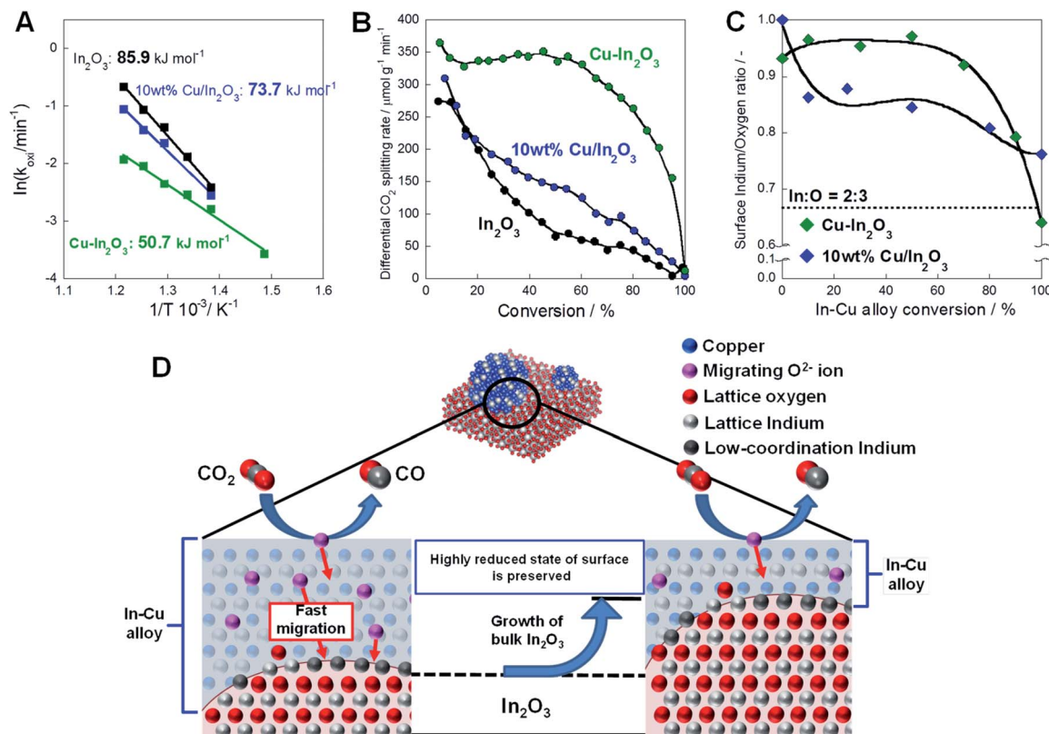
Fig. 6 Kinetics analysis of each oxide in re-oxidation steps. (A) Arrhenius plots for the oxidation of \text{Cu-In}_2\text{O}_3 (derived from \text{Cu}_2\text{In}_2\text{O}_5 ), 10 \text{ wt}\% \text{ Cu/In}_2\text{O}_3 and \text{In}_2\text{O}_3 . (B) Dependence of differential \text{CO}_2 splitting rate on conversion of oxides. (C) Surface \text{In/O} ratios on \text{Cu-In}_2\text{O}_3 and 10 \text{ wt}\% \text{ Cu/In}_2\text{O}_3 during the re-oxidation step. (D) Presumed mechanism of \text{CO}_2 splitting on the reduced \text{Cu-In}_2\text{O}_3 .
