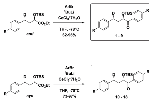
Scheme 3 Synthesis of the syn and anti substrates 1–18.
