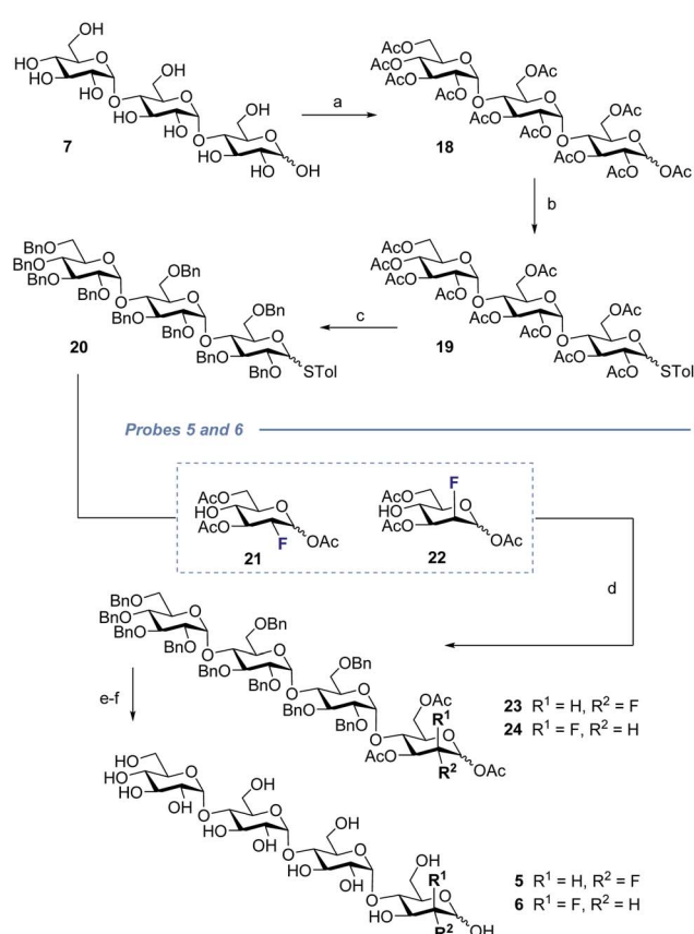
Scheme 2 Preparation of fluorinated maltotetraose cores 5 and 6 . Conditions: (a) \text{Ac}_2\text{O} , DMAP, pyridine, 4 h, RT, 88%. (b) 4-Methylbenzenethiol, \text{BF}_3 \cdot \text{OEt}_2 , \text{CH}_2\text{Cl}_2 , 23 h, RT, 78%. (c) (1) NaOMe, MeOH, 2 h, RT, 91%; (2) NaH, BnBr, TBAI, DMF, 20 h, RT, 77%. (d) NIS, \text{BF}_3 \cdot \text{OEt}_2 , \text{CH}_2\text{Cl}_2 , 15 min, RT, 23%; 21%, 24%, 25%. (e) Pd/C, \text{H}_2 , MeOH, EtOAc, 24 h, RT; (f) NaOMe, MeOH, 8 h, RT, 5: 88%, 6 : 67% over two steps.
