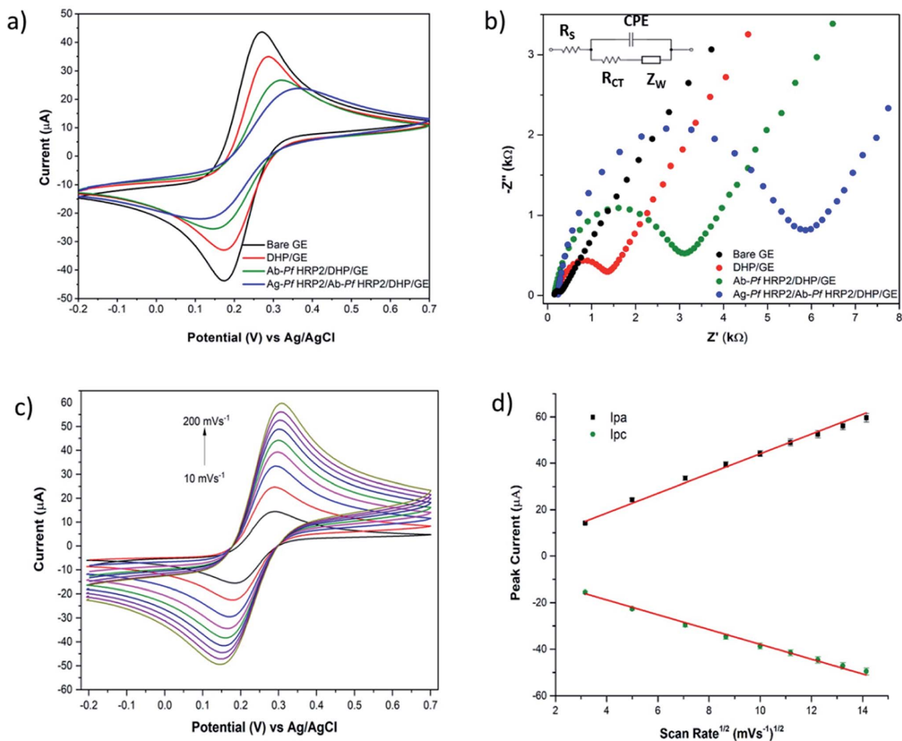
Fig. 3 (a) CVs recorded between -0.2 and +0.7 V at 50 mV s -1 , (b) EIS recorded at +0.23 V by varying the frequency with logarithmic spacing frequency in the range from 10 mHz to 100 kHz, (c) CVs recorded with the immunosensor at different scan rates ( 10 , 25 , 50 , 75 , 100 , 125 , 150 , 175 , 200 mV s -1 ), and (d) plots of peak currents as a function of the square root of the scan rate. All the electrochemical measurements were carried out in 5 mmol L -1 [Fe(CN) 6 ] 4-/3- + 0.1 mol L -1 KCl solution.
