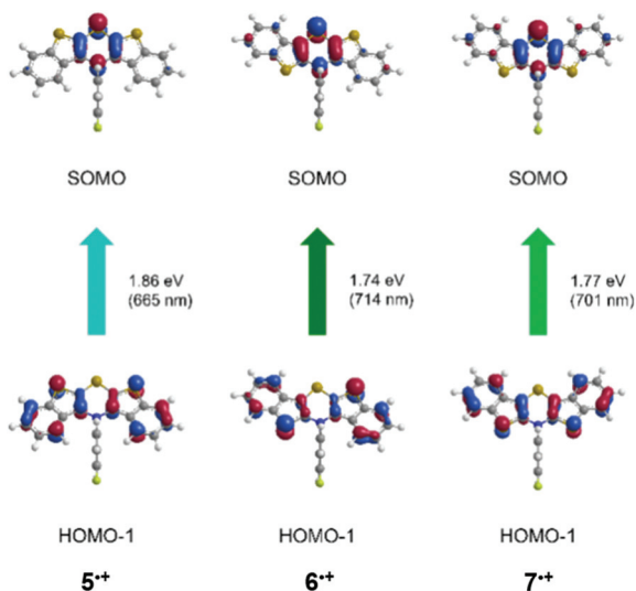
Fig. 11 TDDFT calculated molecular orbital transitions of most bathochromic absorptions of radical cations 5 + , 6 + , and 7 + (uB3LYP/6-311++G**, IEFPCM CH 2 Cl 2 , isosurface value 0.05 a.u.) (For further molecular orbital transitions, see SI).
