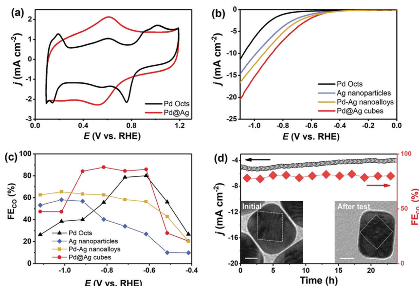
Fig. 6 CO 2 RR performance in CO 2 -saturated 0.5 M KHCO 3 . (a) CV curves without bubbling CO 2 ; (b) polarization curves; (c) FE of CO at various applied potentials; (d) long-term i-t curve and CO FE, along with TEM images before and after electrolysis (scale bar: 20 nm).
