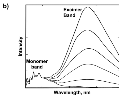
Fig. 2 (a) Mechanism of static and dynamic excimer formation. (b) The monomer and excimer emission band of pyrene at various concentration in cyclohexane.
