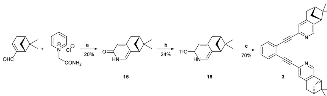
Scheme 2 The synthetic route to ligand 3 . Reagents and conditions: (a) 1. Piperidine, MeOH, reflux, Ar, 2 h. 2. \text{HCONH}_2 , AcOH, 200^\circ\text{C} , 1 h; (b) \text{Tf}_2\text{O} , \text{Et}_3\text{N} , \text{CH}_2\text{Cl}_2 , -50^\circ\text{C} to r.t. 19 h; (c) 1,2-diethynylbenzene, Pd( \text{PPh}_3 ) _2\text{Cl}_2 , CuI, \text{PPh}_3 , DIEA, MW 110^\circ\text{C} , 15 min. For details, see the ESI.†
