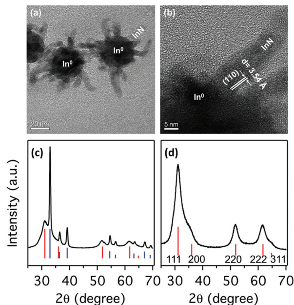
Fig. 22 TEM images of the NPs. (a) Overview of the as prepared sample, showing the \text{InN} branches stemming out of larger \text{In}(0) NPs. (b) HRTEM image of one of the \text{InN} branches in (a) at the surface of the \text{In}(0) nanoparticle. XRD pattern for the (c) as-prepared sample and (d) acid treated sample. The vertical lines show the XRD patterns of bulk zinc blende- \text{InN} (red) and tetragonal \text{In}(0) (blue). Reprinted with permission from ref. 176. Copyright 2016 American Chemical Society.
