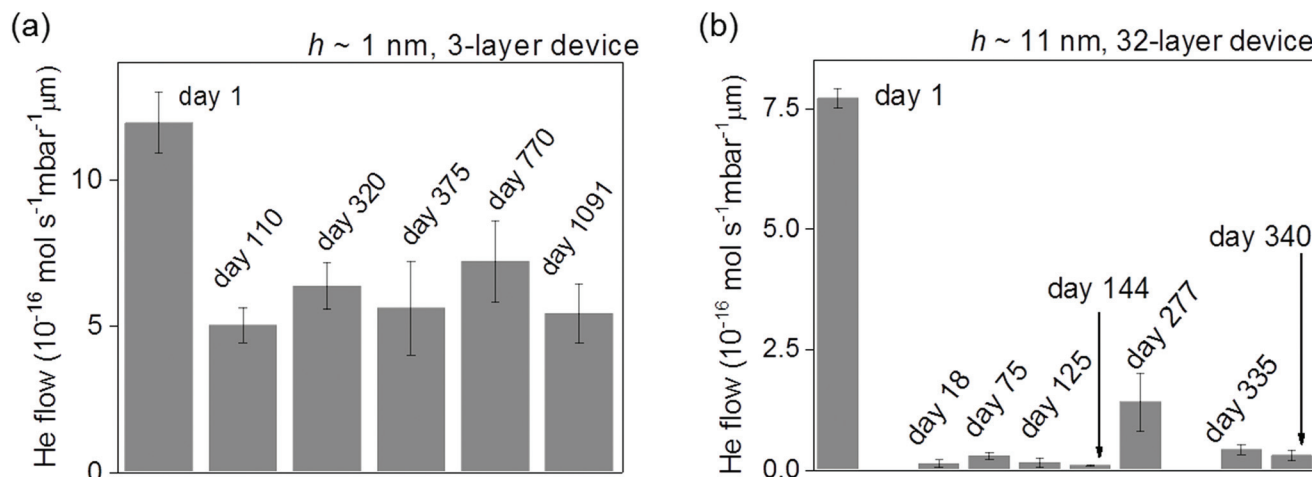
Fig. 2 He flow through Å-channel devices with heights, (a) h \sim 1 nm (3-layer graphene spacer) and (b) h \sim 11 nm (32-layer graphene spacer) monitored for over a duration of three years and one year, respectively. The bars represent He flows arbitrarily checked on different days through the same device when it was stored under charcoal. The devices were annealed before each measurement. Error bars are from two measurements on the same device.
