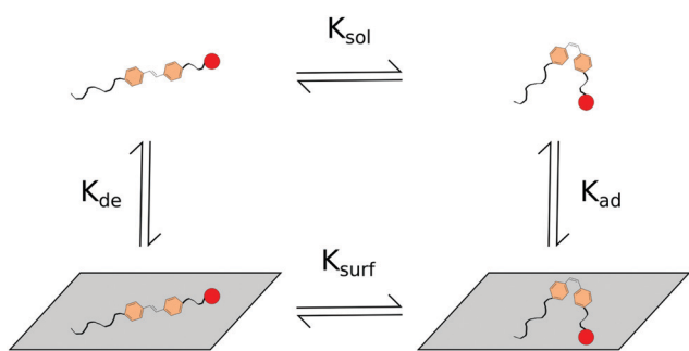
Fig. 8 Scheme for the proposed interactions of photo-responsive components interacting with surfaces.
