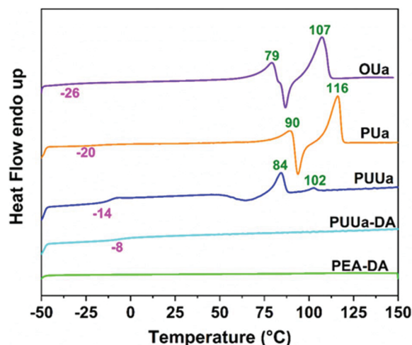
Fig. 5 DSC curves of oligourea (OUa), polyurea (PUa), polyurethane-urea (PUUa), the polyurethane-urea Diels–Alder adduct (PUUa-DA) and the poly(propylene glycol) bis(2-aminopropyl ether) Diels–Alder adduct (PEA-DA) from the second heating scan.
