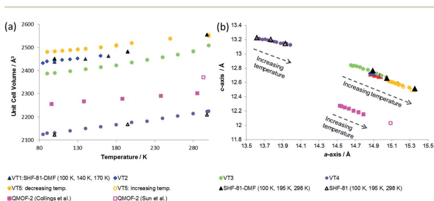
Fig. 7 (a) Unit cell volume as a function of temperature and (b) lattice parameters during in situ SCXRD ( VT2 , VT3 , SHF-81-DMF ; VT4 , SHF-81 ) and PXRD ( VT5 , SHF-81-DMF ) studies. Data for full crystal structure determinations of SHF-81-DMF and SHF-81 at different temperatures are included, as are data for the previously reported VT-NPD study 31 of desolvated QMOF-2 and single-crystal structure determination 45 of solvated QMOF-2 (note: the linear NTE behaviour of QMOF-2 was studied in the temperature range 12–285 K; data for the two studies conducted below 80 K are excluded from (a) for clarity of presentation, but studies over the full temperature range are included in (b)).
