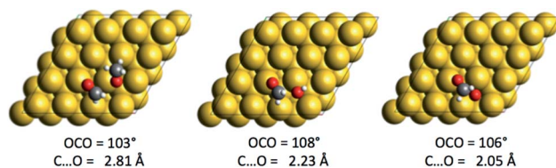
Fig. 3 Structures of the three transition states associated with the A_{\text{N}2} of O, OH and CH 3 O onto CH 2 O.
