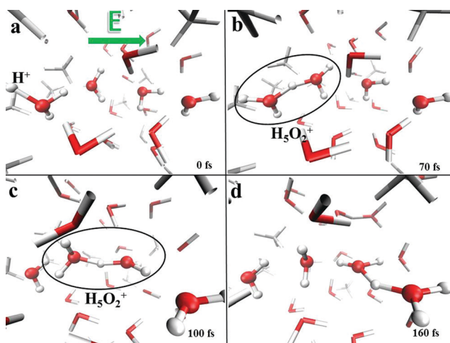
Fig. 10 Proton transfer in a liquid methane–water mixture induced by a static and homogeneous electric field. Once a series of H-bonded “water wires” with dipoles heading towards the field direction are formed (a), the formation of a Zundel cation ( \text{H}_5\text{O}_2^+ ) can occur (b). If the field strength is intense enough, the Zundel cation suddenly ( \sim 30 \text{ fs} ) propagates (c). Migration of the proton along the field direction via the Grotthuss mechanism partially reverts some of the molecular dipoles (d).
