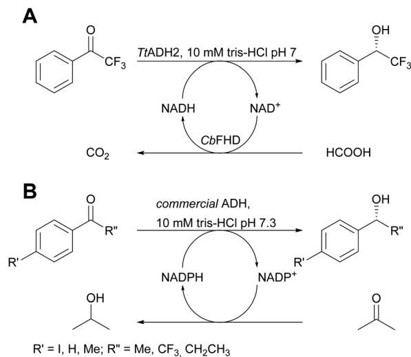
Scheme 2 (A) Asymmetric reduction of 2,2,2-trifluoro-1-phenylethanol-1-one catalysed by TtADH2 with external cofactor recycling by CbFDH ; (B) asymmetric reduction of ketones with internal cofactor recycling.
