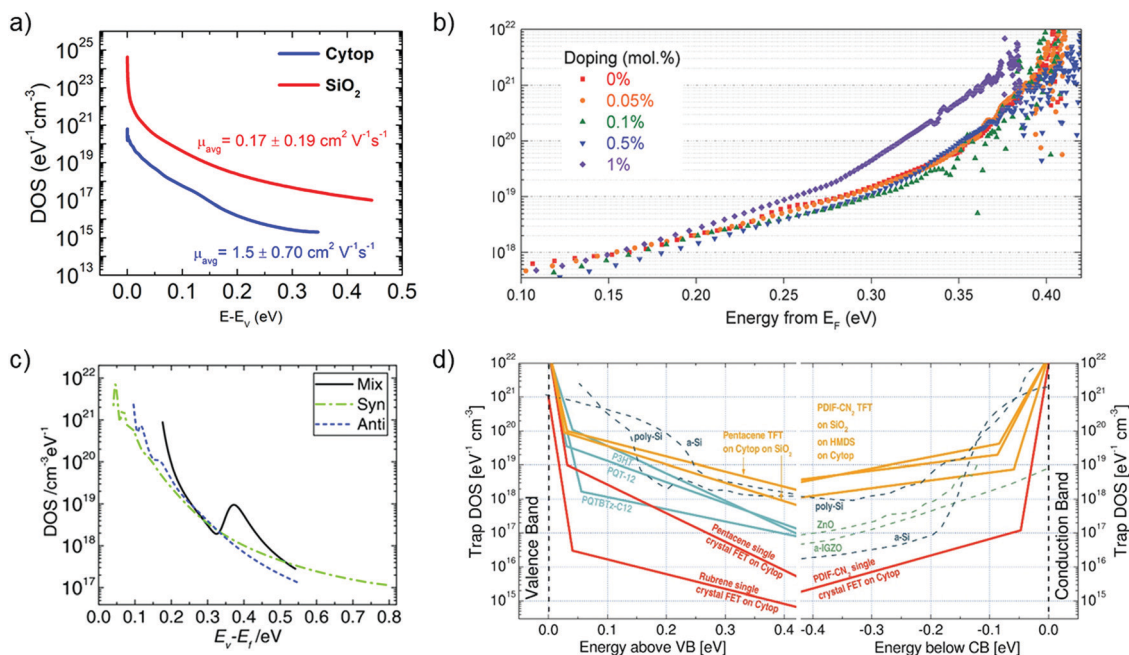
Fig. 10 (a) Comparison of the interfacial trap DOS spectrum for diF-TES ADT films with Cytop (blue) and \text{SiO}_2 (red) dielectrics evaluated using Grünewald's model. The value of mobility is listed in the inset. Adapted with permission from ref. 97, Copyright 2015, AIP Publishing LLC. (b) Effect of p-doping on the trap DOS of OSC/polymer blend OFETs evaluated using Grünewald's model. Reproduced with permission from ref. 198, Copyright 2017, Wiley-VCH. (c) Effect of isomer purity of diF-TES ADT on the trap DOS spectrum determined using Method II by Kalb et al. Broken green and blue curves represent trap DOS of pure syn - and anti -isomers respectively while the solid black lines represent that of the mix sample for reference. Reproduced with permission from ref. 205, Copyright 2017, Wiley-VCH. (d) Comparison of the interfacial trap DOS for several organic and inorganic FETs calculated using the numerical method by Oberhoff et al. Reproduced with permission from ref. 208, Copyright 2010, American Physical Society.
