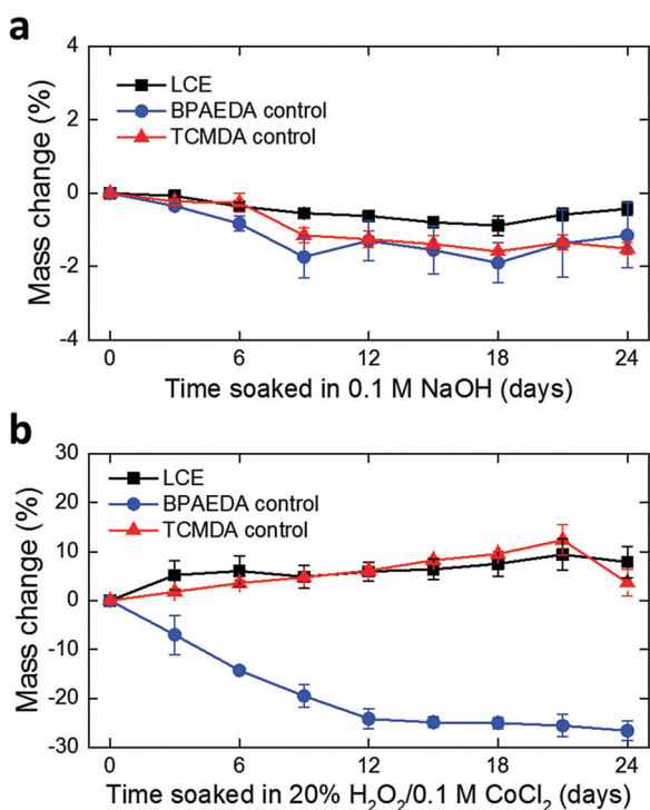
Fig. 2 Monitoring of mass change in LCE and control films over 24 days in (a) 0.1 M NaOH (mean \pm SD, n = 4 ) and (b) 20% \text{H}_2\text{O}_2 /0.1 M \text{CoCl}_2 (mean \pm SD, n = 4 ), both at 37 °C.
