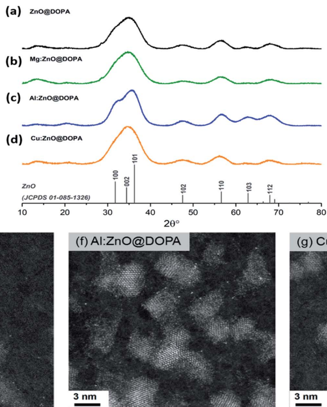
Fig. 1 Powder XRD patterns and HAADF-STEM images of (a) ZnO@DOPA, (b) & (e) Mg:ZnO@DOPA, (c) & (f) Al:ZnO@DOPA and (d) & (g) Cu:ZnO@DOPA. Patterns are indexed against ZnO as grey vertical bars (JCPDS 01-085-1326). All scale bars in the STEM images are 3 nm.
